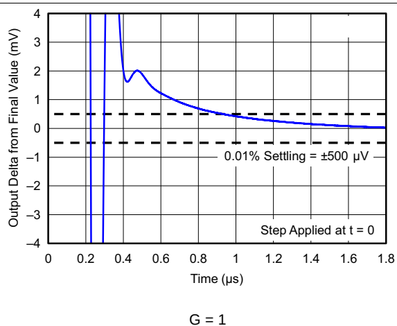
Figure 28. Settling Time (5-V Positive Step)
