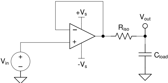
Figure 38. Extending Capacitive Load Drive With the TLVx197-Q1
