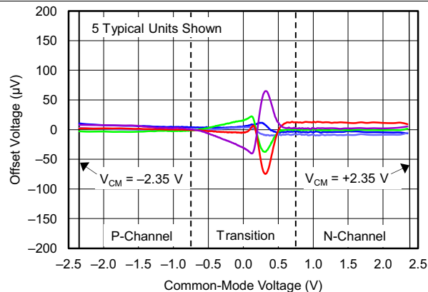
Figure 1. Offset Voltage vs Common-Mode Voltage
