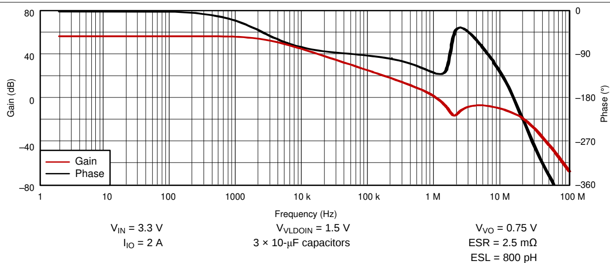
Figure 25. DDR3 Design Example Bode Plot
