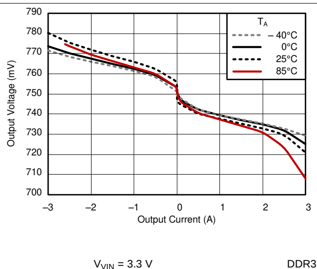
Figure 26. Load Regulation
