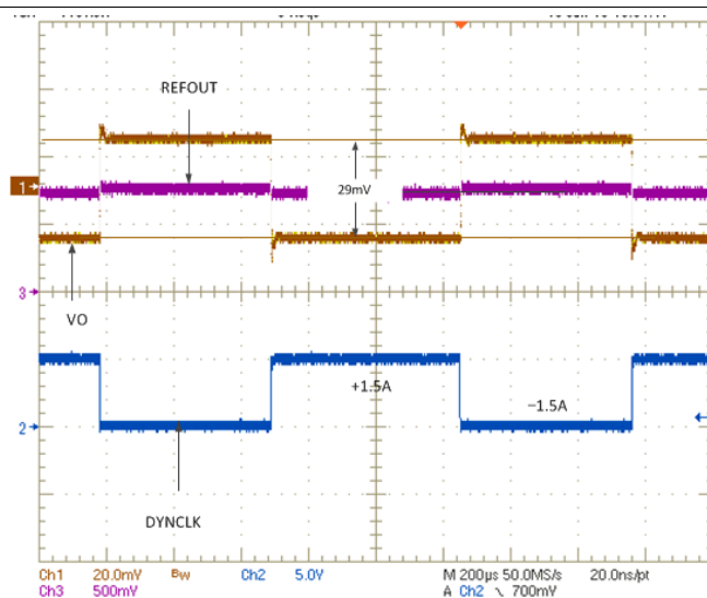
Figure 27. Transient Waveform
