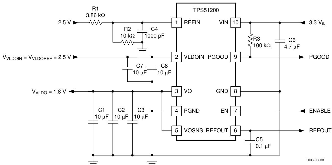
Figure 32. 3.3- V_{IN} , LDO Configuration
