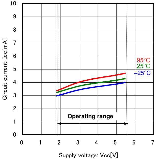
Figure 4 Circuit current
