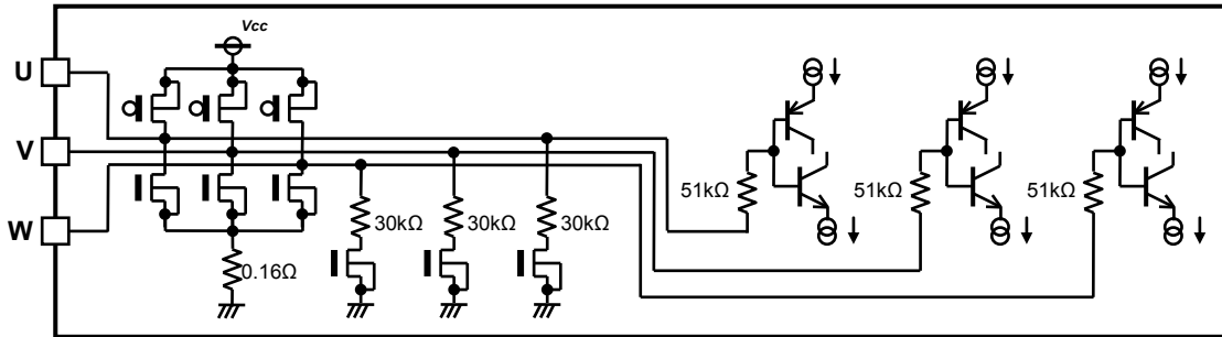
Figure 30. I/O equivalent circuits
