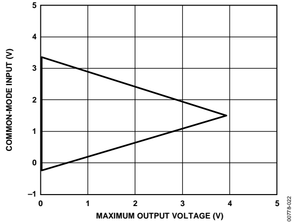
Figure 34. Common-Mode Input vs. Maximum Output Voltage, G = 1 , +V_S = 5 \text{ V} , -V_S = 0 \text{ V} , R_L = 100 \text{ k}\Omega , N-8 Package Option
