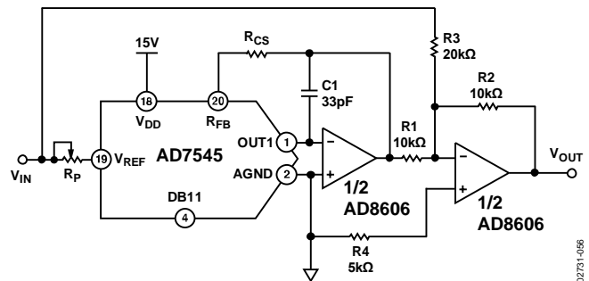
Figure 59. Bipolar Operation
