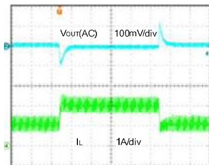
Load Transient
