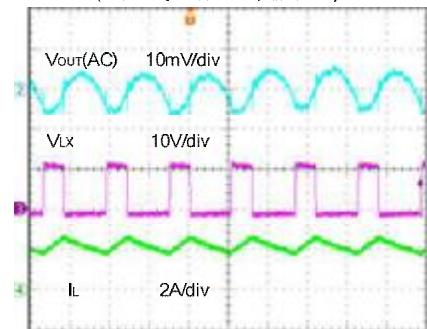
Output Ripple
