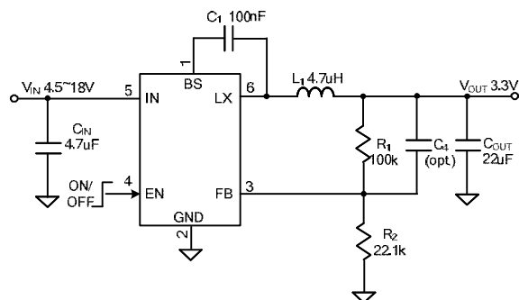
Figure 1. Schematic Diagram
