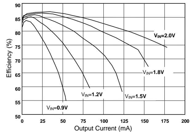
Fig. 27 AIC1642-33 Efficiency (L=100μH, CD54)
