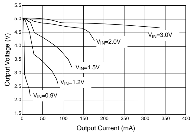
Fig. 55 AIC1642-50 Load Regulation (L=47μH CD54)
