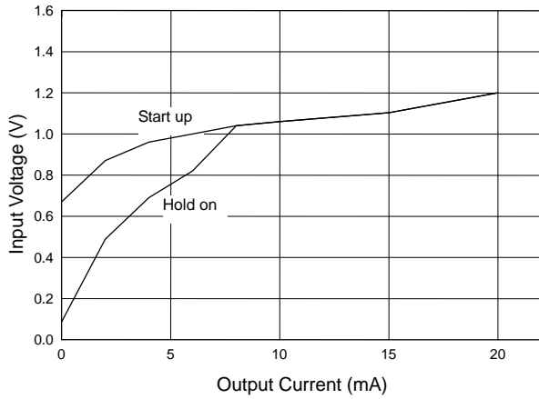
Fig. 40 AIC1642-37 Start-up & Hold-on Voltage (L=100μH)
