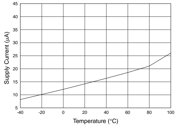
Fig. 25 AIC1642-30 Supply Current vs. Temperature
