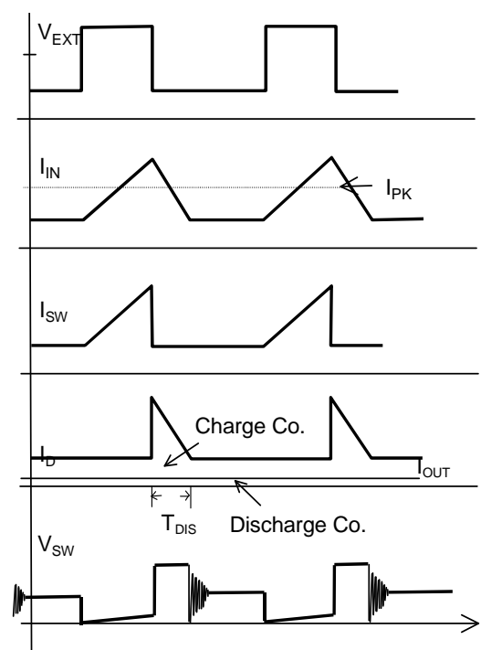
Discontinuous Conduction Mode
