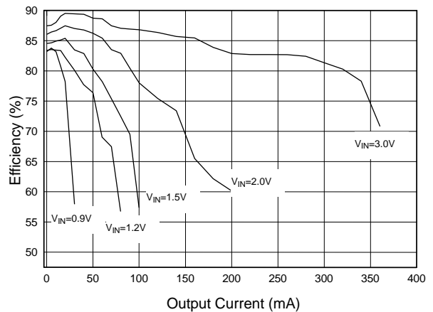
Fig. 45 AIC1642-45 Efficiency (L=100μH)
