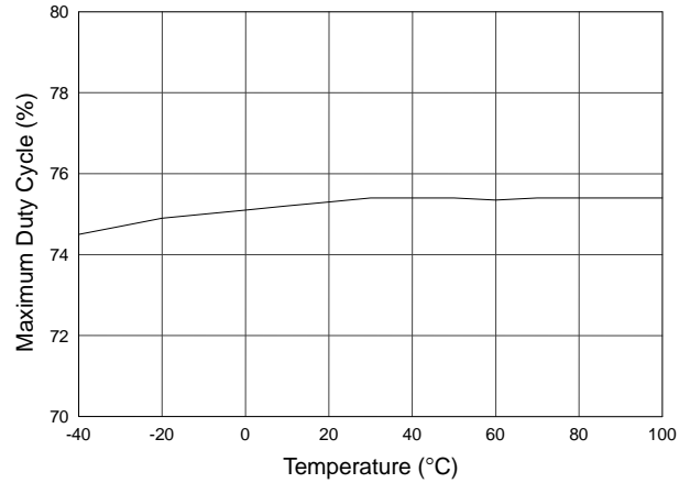
Fig. 23 AIC1642-30 Maximum Duty Cycle vs. Temperature
