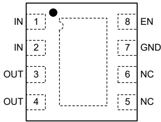
TDFN-3x3-8L
