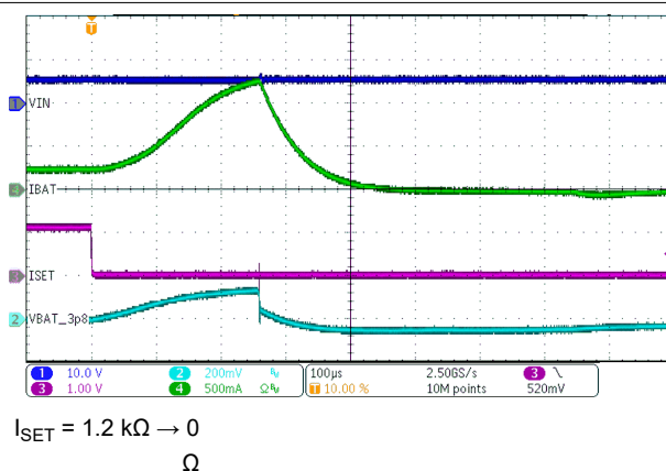
Figure 8-9. OUT Transient Response
