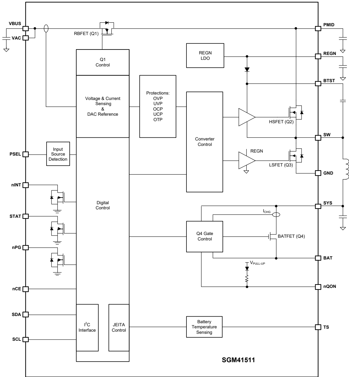
Figure 2. Block Diagram
