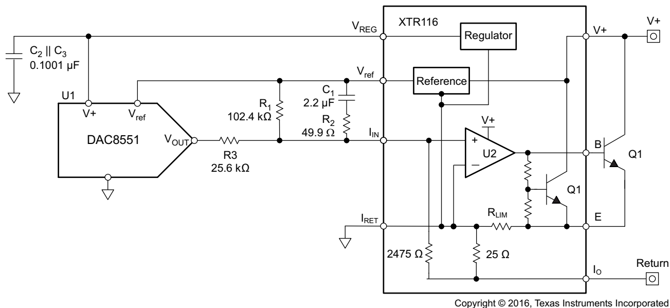
Figure 52. Loop-Powered Transmitter
