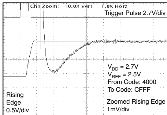
Figure 38. Half-Scale Settling Time: 2.7-V Rising Edge
