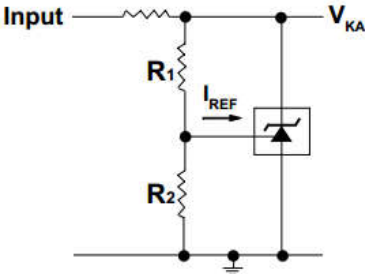
(Figure2. Test circuit for V_{KA}>V_{REF} )
