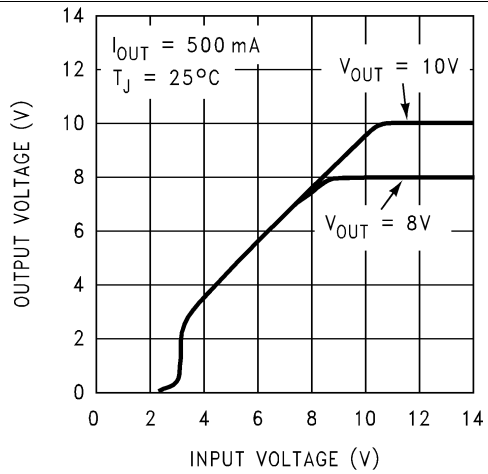
Figure 14. Low-Voltage Behavior
