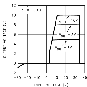
Figure 25. Output at Voltage Extremes
