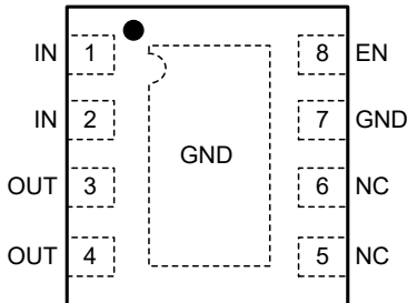
TDFN-3x3-8L
