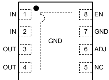
TDFN-3x3-8L
