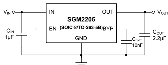
Figure 2. Low Noise Regulator (Fixed Voltage Version)
