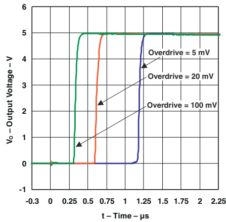
图 7-5. Response Time for Various Overdrives Positive Transition
