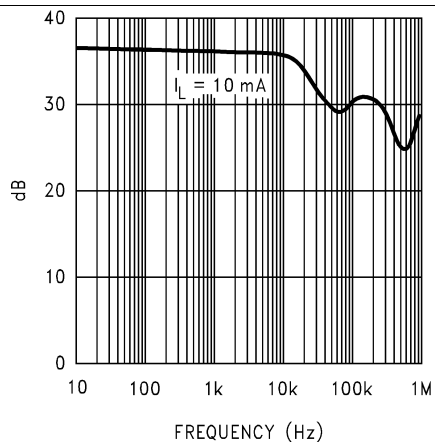
Figure 7. Ripple Rejection
