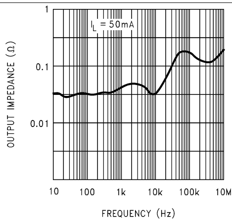
Figure 8. Output Impedance
