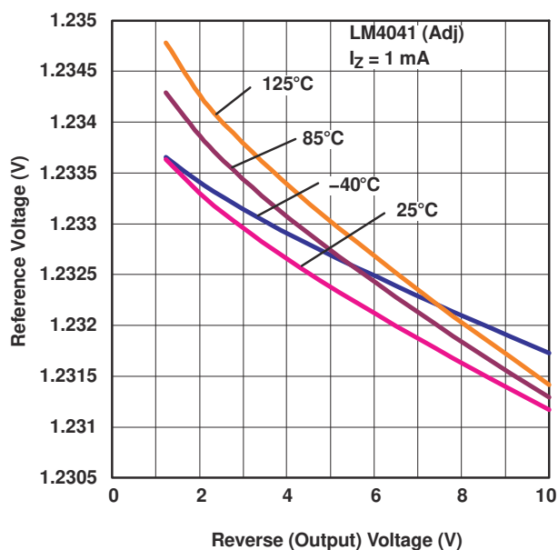
图 13-4. Reference Voltage vs Reverse (Output) Voltage (for Different Temperatures)
