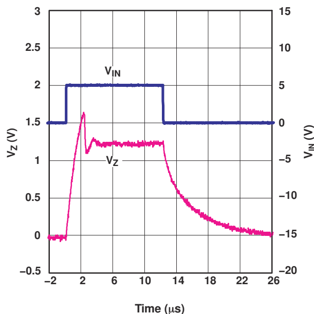
图 13-3. Start-Up Characteristics
