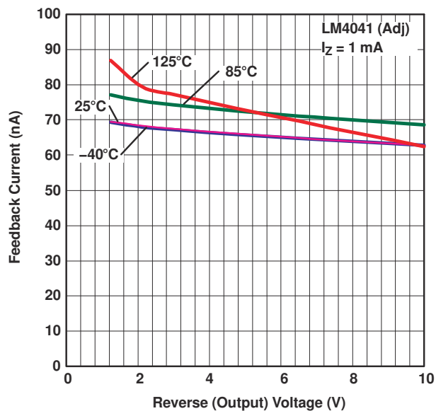
图 13-6. Feedback Current vs Reverse (Output) Voltage (for Different Temperatures)
