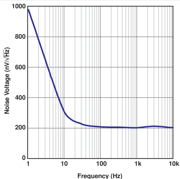
图 13-2. Noise Voltage vs Frequency
