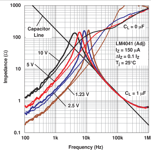
图 13-8. Output Impedance vs Frequency
