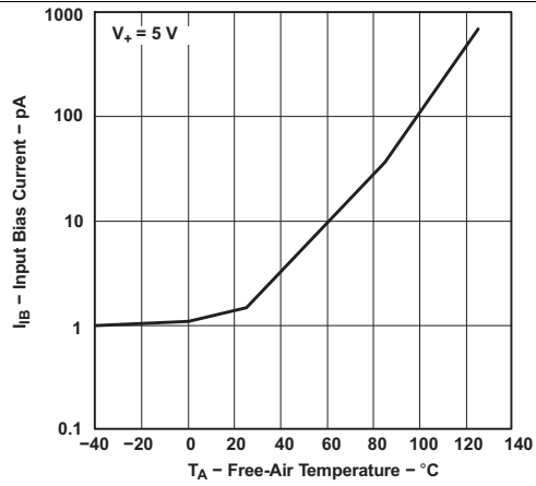
Figure 2. Input Bias Current vs Temperature
