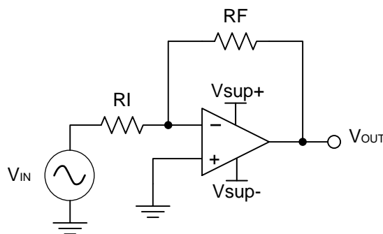
Figure 37. Application Schematic
