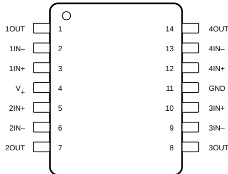
Pin Functions: LMV344
