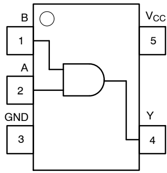
(SC-88A / TSOP-5 / SC-74A)
