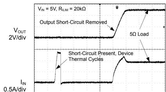
Short-Circuit to Full-Load Recovery Response
