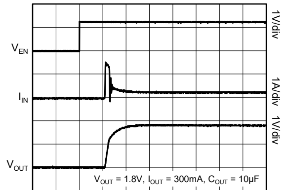
Time (50 \mu\text{s}/\text{div} )
