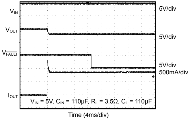
Resistance Load Inrush Response (SGM2588A/B/G)
