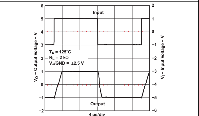
Figure 30. Large-Signal Noninverting Response
