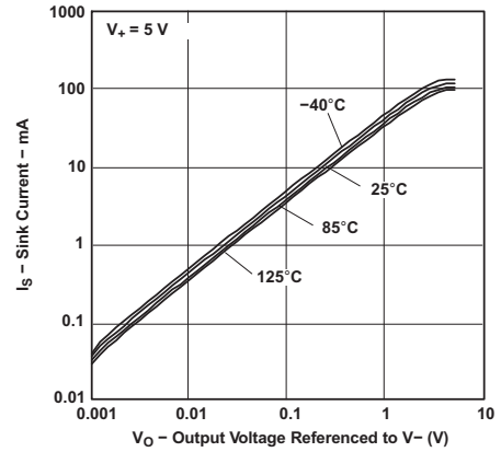
Figure 8. Sink Current vs Output Voltage
