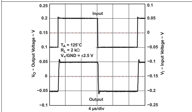
Figure 29. Small-Signal Noninverting Response
