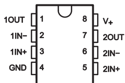
TLV342 D or DGK Package 10-Pin SOIC or VSSOP Top View
