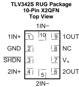
Pin Functions: TLV342S
