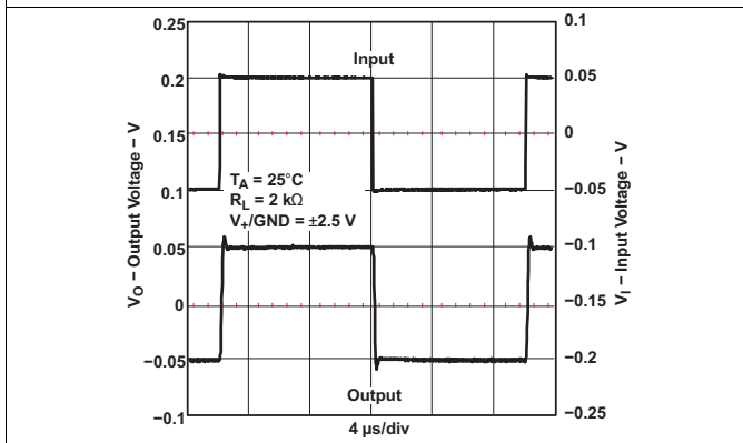
Figure 27. Small-Signal Noninverting Response
