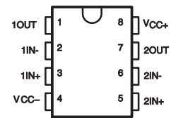
DCT OR DDU PACKAGE (TOP VIEW)
