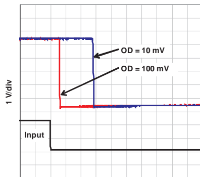
PROPAGATION DELAY TIME, HIGH TO LOW V_{CC} = 5\text{ V}
