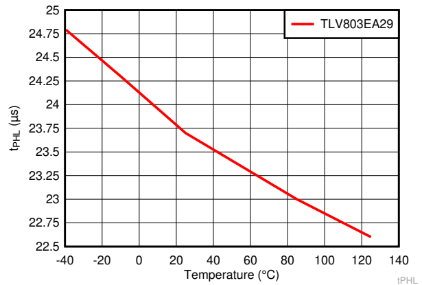
Figure 7-24. High-to-Low Propagation Delay Verses Temperature for TLV803EA29
