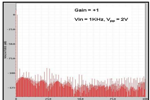
THD+Noise, Gain = +1, V_{IN} = 1\text{kHz} , V_{PP} = 2\text{V}
