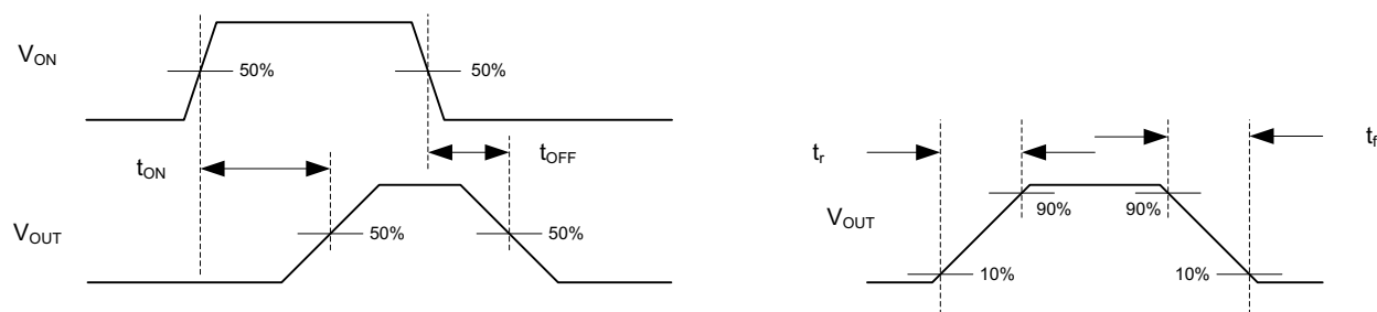
t_{ON}/t_{OFF} WAVEFORMS
