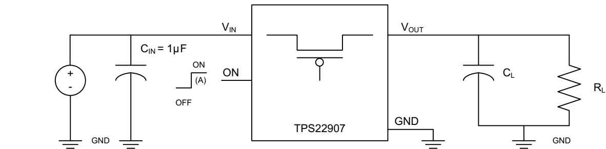
TEST CIRCUIT
