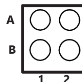
YZT Package 4-Pin DSBGA (Bump View)
