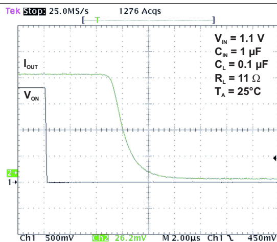
Figure 17. t_{OFF} Response
