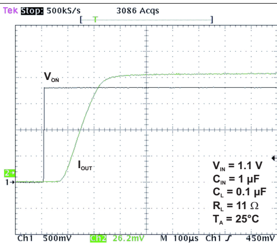
Figure 16. t_{ON} Response
