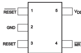
Figure 6-3. 5-Pin SOT-23 TPS3825: DBV Package (Top View)
