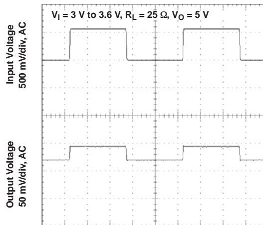
Figure 20. TPS61071 Line Transient Response
