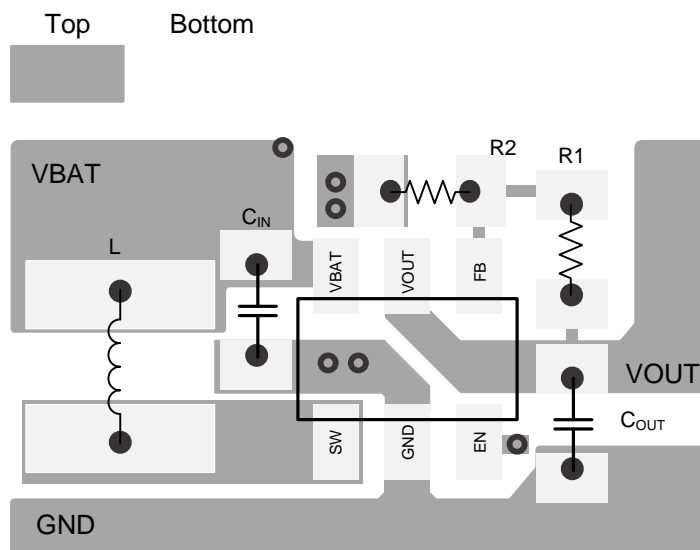
Figure 30. PCB Layout
