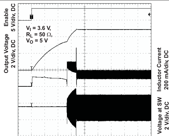
Figure 22. TPS61070 Start-Up After Enable
