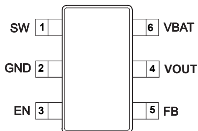
DDC Package 6 Pins Top View
