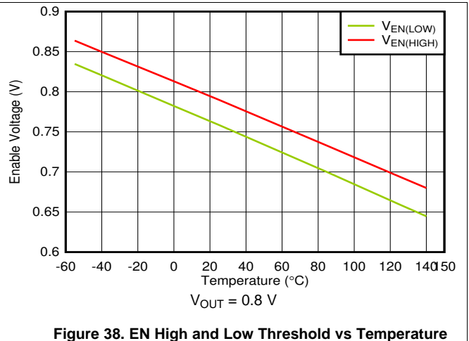
Figure 38. EN High and Low Threshold vs Temperature
