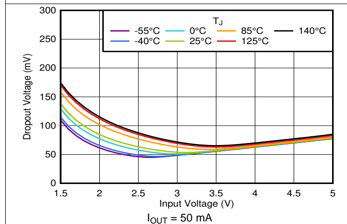
Figure 35. Dropout vs V_{IN} and Temperature
