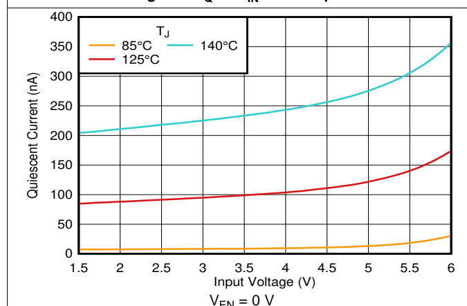
Figure 11. I_{SHDN} vs V_{IN} and Temperature
