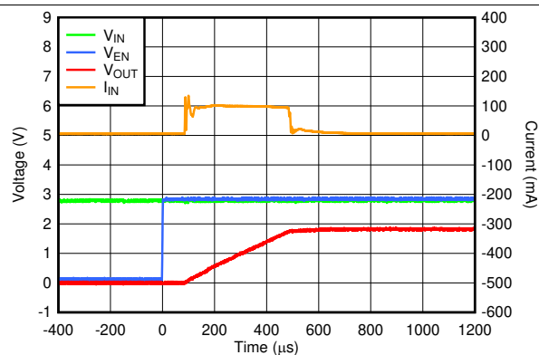
Figure 56. Startup Inrush Current With C_{OUT} = 22\text{ }\mu\text{F}
