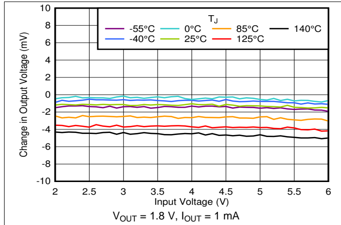
Figure 25. Line Regulation vs V_{IN} and Temperature
