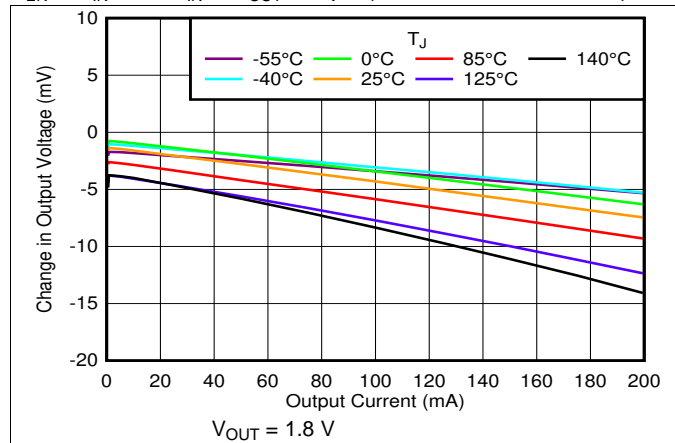
Figure 31. Load Regulation vs V_{IN} and Temperature
