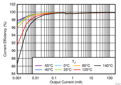
Figure 62. Current Efficiency vs I_{OUT} and Temperature
