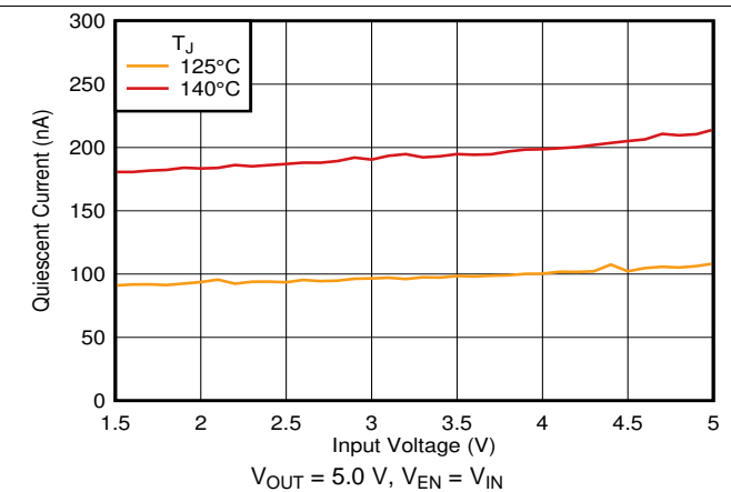
Figure 8. I_Q in Dropout vs V_{IN} and Temperature
