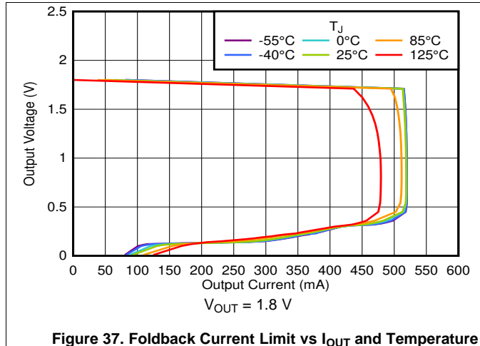
Figure 37. Foldback Current Limit vs I_{OUT} and Temperature
