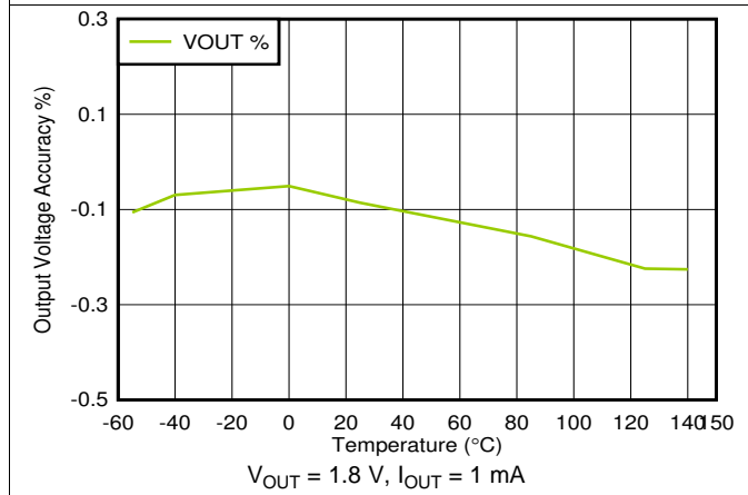
Figure 27. Output Accuracy vs Temperature
