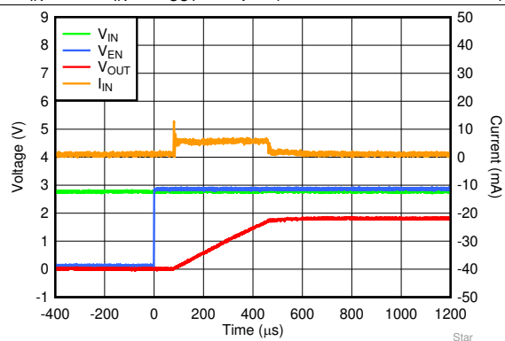
Figure 55. Startup Inrush Current With C_{OUT} = 1\text{ }\mu\text{F}
