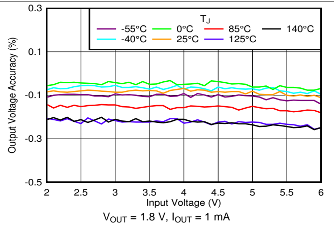
Figure 26. Output Accuracy vs V_{IN} and Temperature
