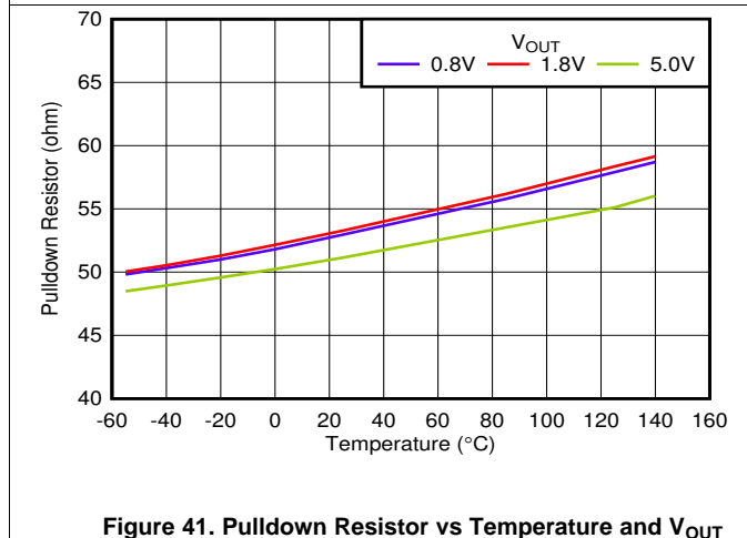
Figure 41. Pulldown Resistor vs Temperature and V_{OUT}
