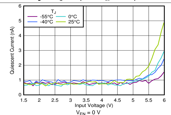
Figure 10. I_{SHDN} vs V_{IN} and Temperature
