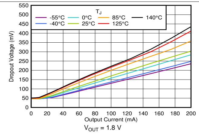
Figure 32. Dropout vs I_{OUT} and Temperature
