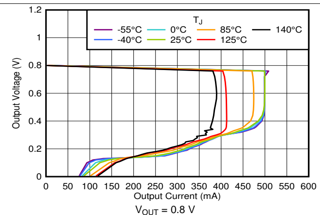
Figure 36. Foldback Current Limit vs I_{OUT} and Temperature
