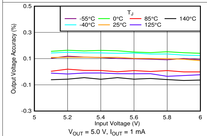
Figure 29. Output Accuracy vs V_{IN} and Temperature
