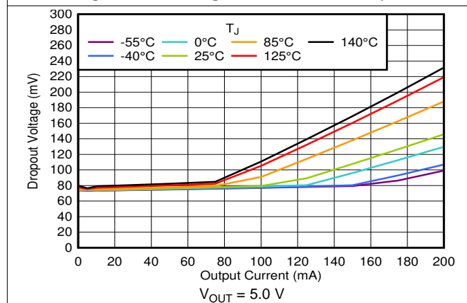
Figure 33. Dropout vs I_{OUT} and Temperature
