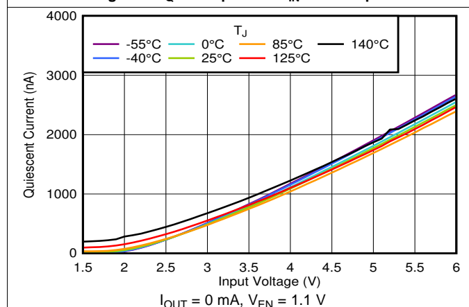
Figure 9. I_Q vs V_{IN} and Temperature
