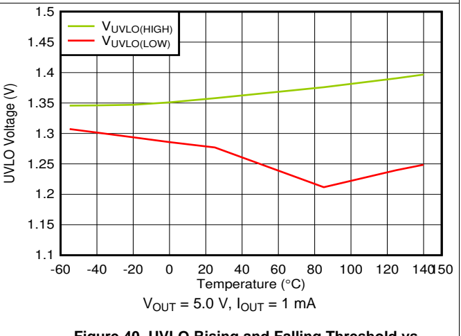
Figure 40. UVLO Rising and Falling Threshold vs Temperature
