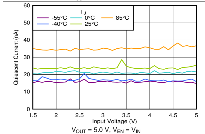
Figure 7. I_Q in Dropout vs V_{IN} and Temperature
