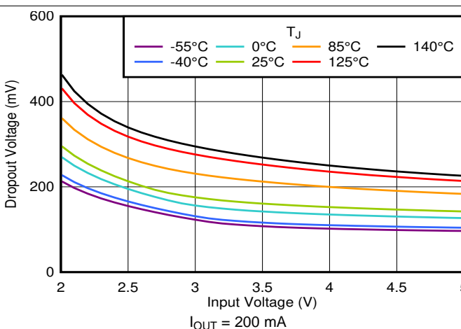
Figure 34. Dropout vs V_{IN} and Temperature
