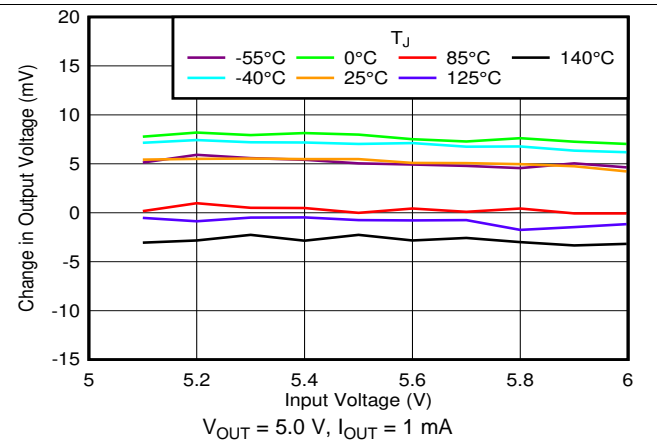
Figure 28. Line Regulation vs V_{IN} and Temperature
