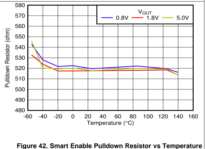
Figure 42. Smart Enable Pulldown Resistor vs Temperature and V_{OUT}
