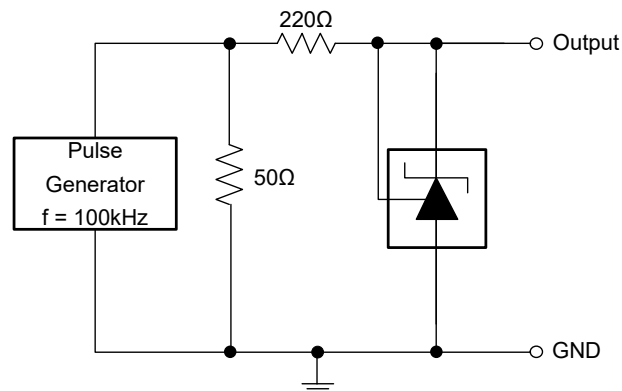
Figure 5. Test Circuit for Pulse Response
