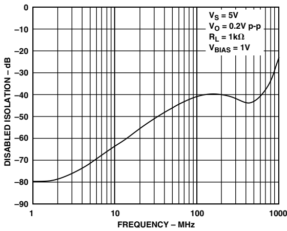
TPC 27. Disabled Output Isolation Frequency Response
