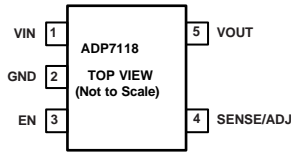
Figure 4. 5-Lead TSOT Pin Configuration
