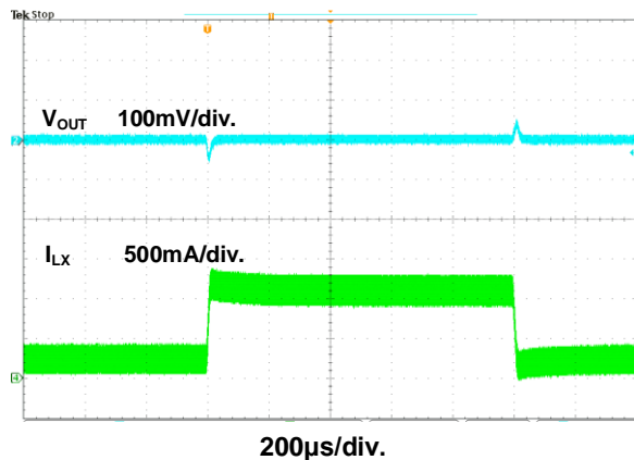
Figure 17. Load Transient Waveform
