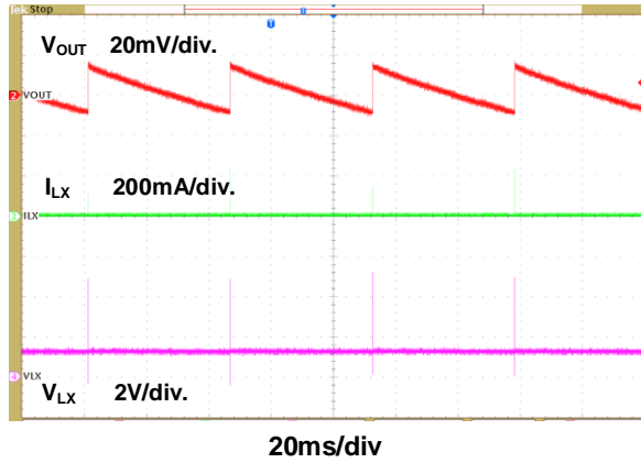
Figure 16. Steady State Waveform
