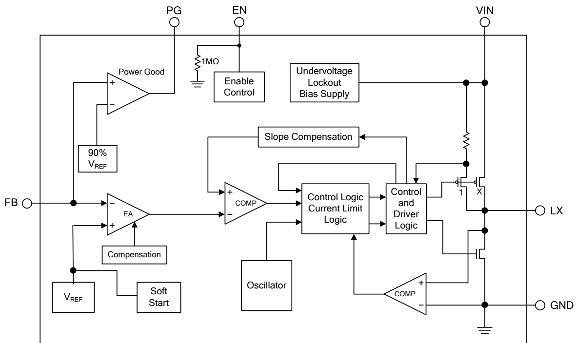
Figure 3. Block Diagram of FP6378A
