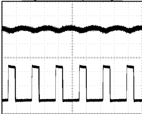
V_{\text{IN}} = 12\text{V} , V_{\text{OUT}} = 3.3\text{V} , I_{\text{OUT}} = 200\text{ mA} Top trace: V_{\text{OUT}} , 10 mV/div, AC Coupled Bottom trace: SW, 5V/div, DC Coupled T = 1\ \mu\text{s/div}
