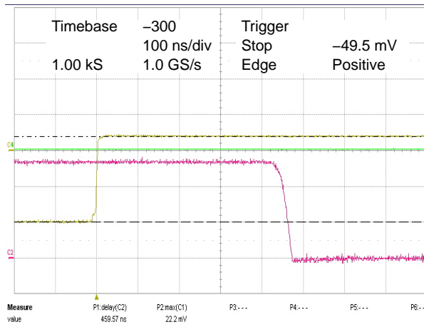
Figure 11. 20 mV Overdrive
