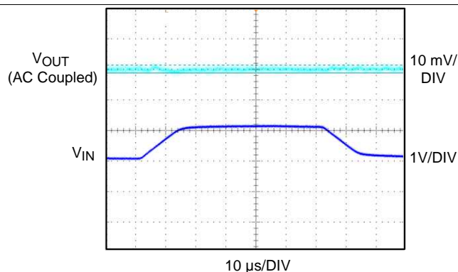
Figure 8. Line Regulation
