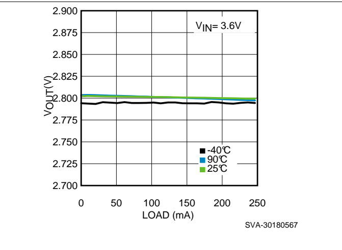
Figure 6. Load Regulation
