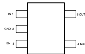
DBV Package 5-Pin SOT-23 Top View
