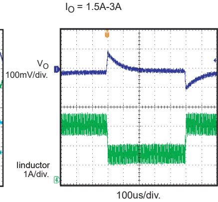
Loop Response
