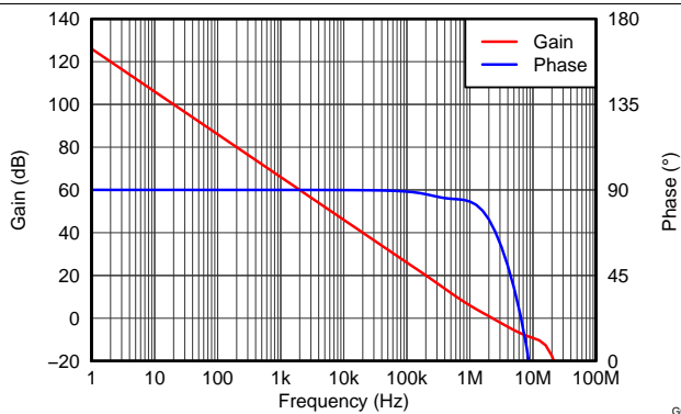
Figure 20. Open-Loop Gain and Phase vs Frequency
