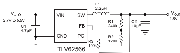
Figure 29. TLV62566 1.8-V Output Application
