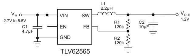
Figure 25. TLV62565 1.2-V Output Application
