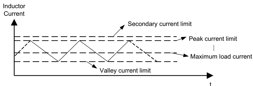
Figure 24. Switch Current Limit
