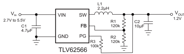
Figure 28. TLV62566 1.2-V Output Application
