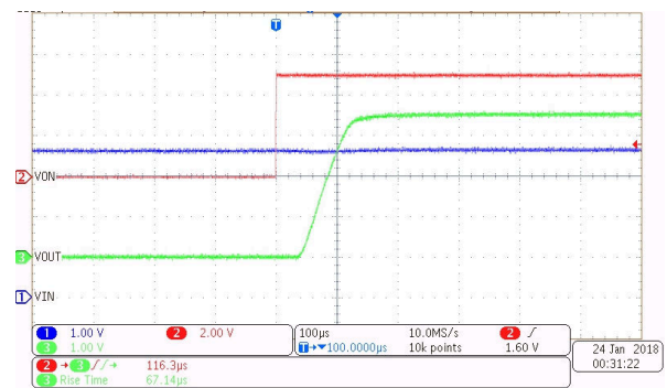
Figure 7-10. Turn-On at 3.6 V (CT = Open)
