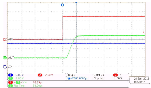
Figure 7-8. Turn-On at 5 V (CT = Open)
