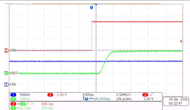
Figure 7-12. Turn On at 1 V (CT = Open)
