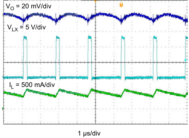
Figure 8-9. TPS562201 Output Voltage Ripple, I_{OUT} = 2 A
