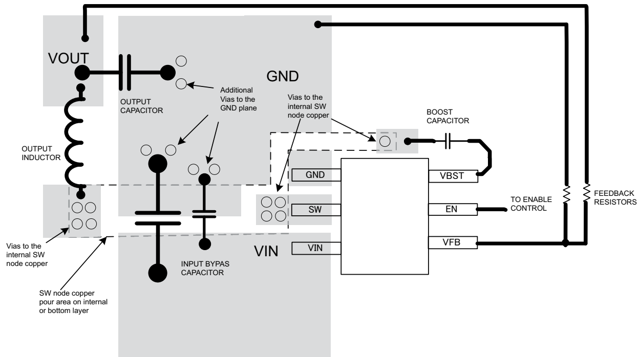
Figure 10-1. TPS562201 and TPS562208 Layout
