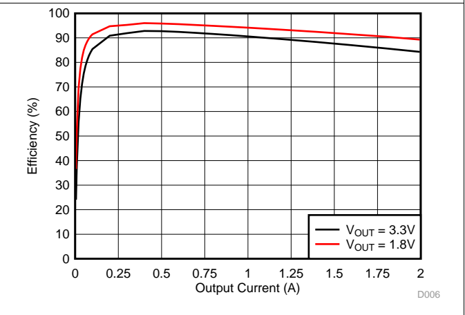
Figure 6. Efficiency vs Output current ( V_I = 5 V )
