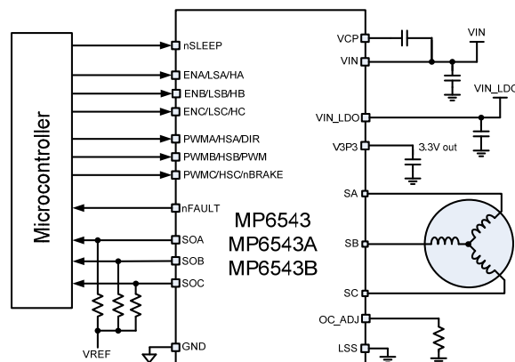
MP6543/6543A/6543B Typical Application Circuit (QFN-24 3mmx4mm)
