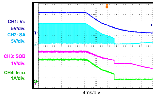
Power Ramp-Down
