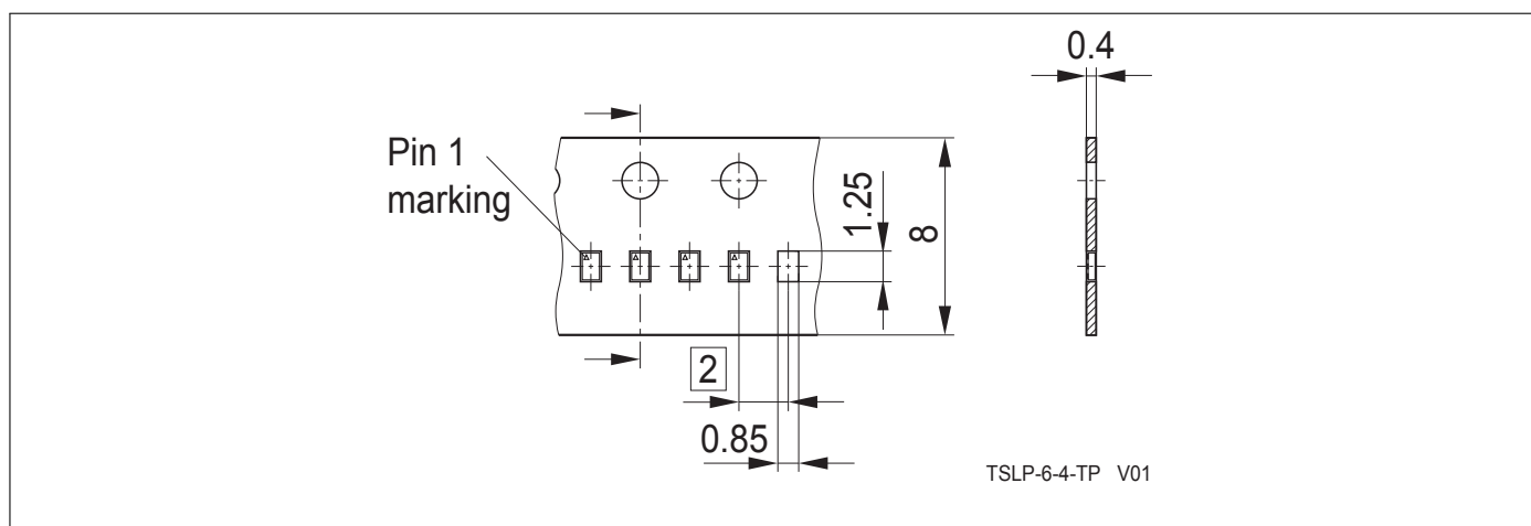
Figure 6: Tape Drawing for TSLP-6-4
