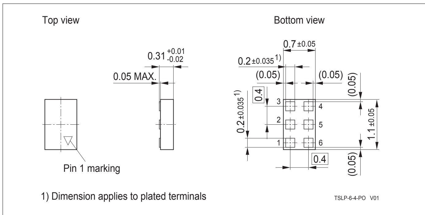
Figure 3: Package Outline
