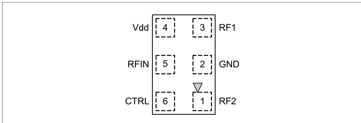
Figure 2: Pin Configuration
