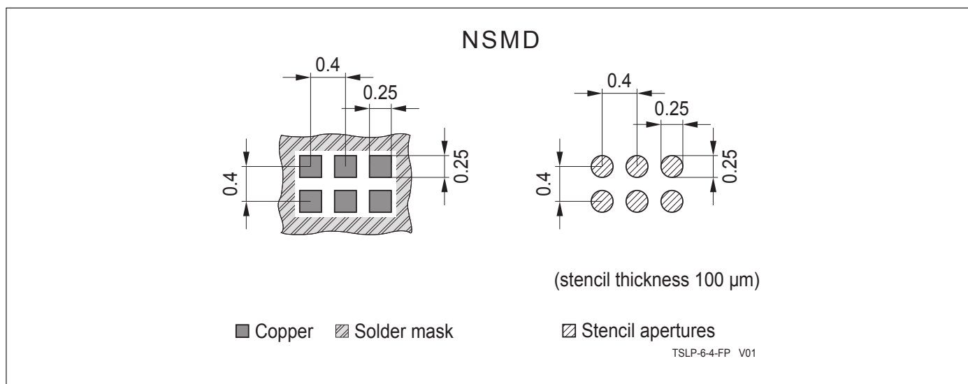
Figure 4: Footprint
