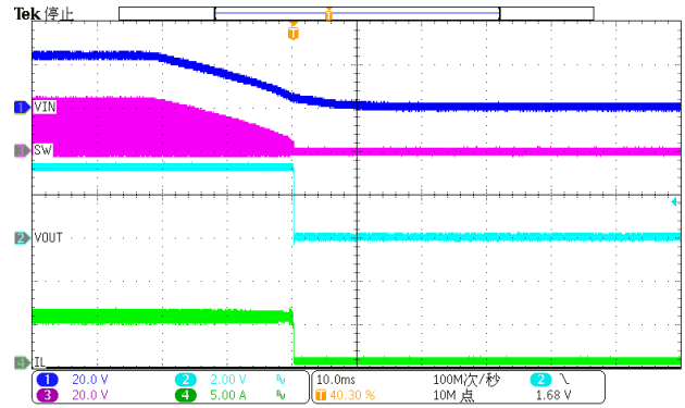
Figure 14. Power down(Iload=5A)
