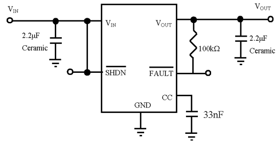
Fig. 1. EMP8965 with Fault. Fixed output version.
