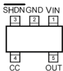
SOT-23-5(Top View)
