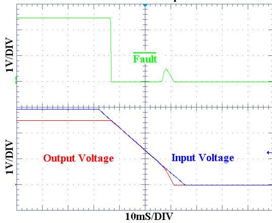
Power-Down Response
