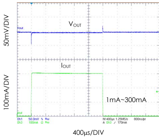
Load Transient
