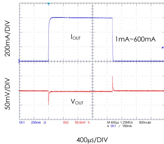
Load Transient
