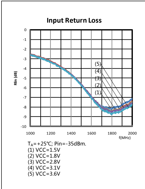
Figure 19. Input return loss as a function of frequency; typical value
