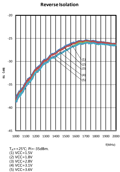
Figure 25. Reverse Isolation as a function of frequency; typical values
