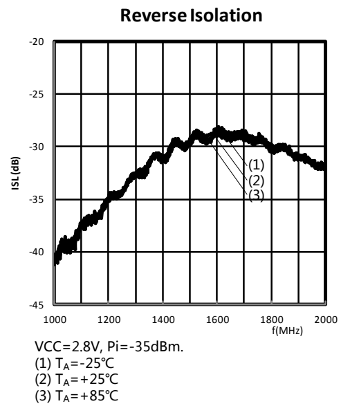
Figure 24. Reverse Isolation as a function of frequency; typical values;
