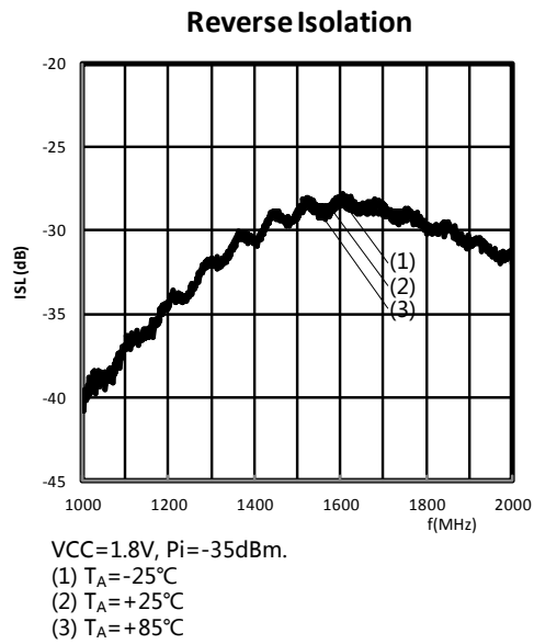
Figure 23. Reverse Isolation as a function of frequency; typical values;
