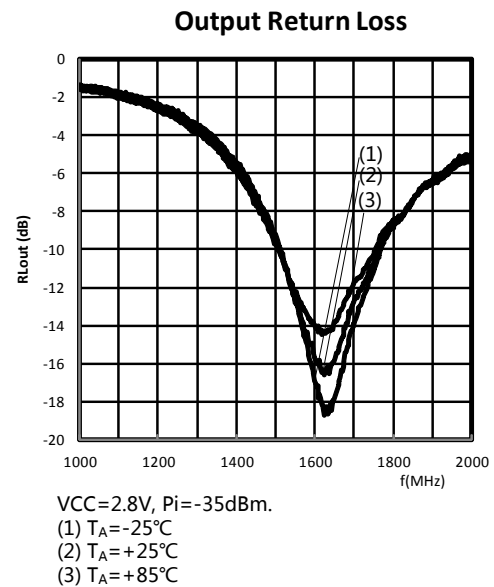
Figure 22. Output Return Loss as a function of frequency; typical values
